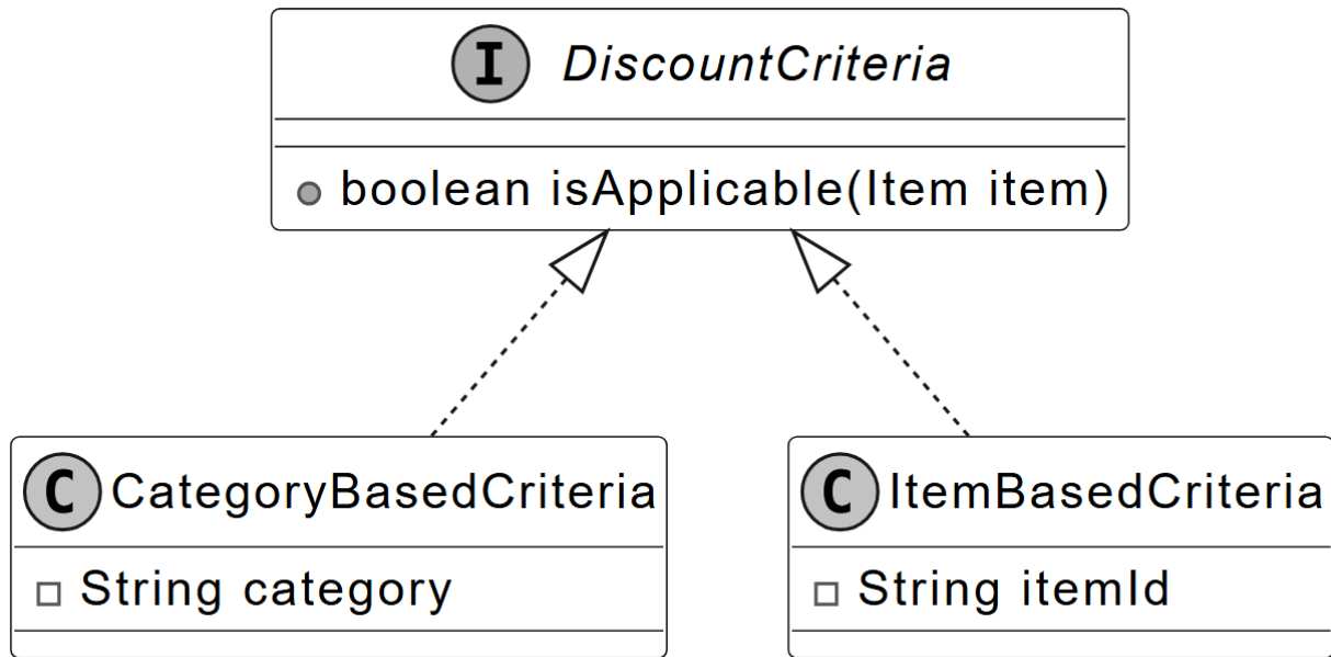
DiscountCriteria interface and concrete classes
