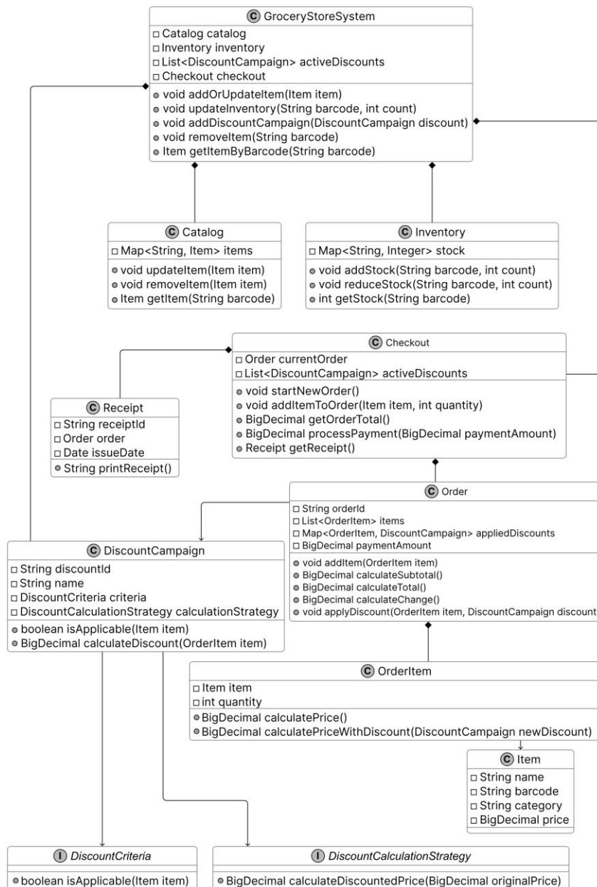
Class Diagram of Grocery Store System
