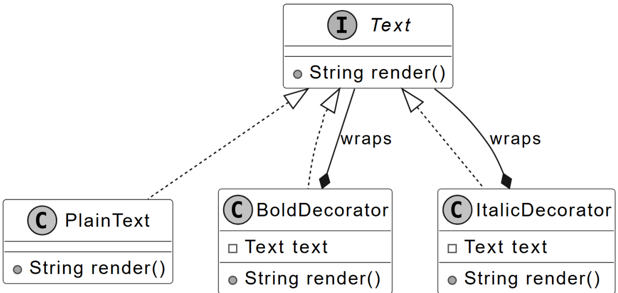
Text interface and concrete classes
